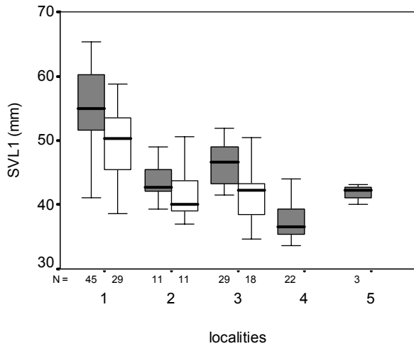
FIG. 5. Back-calculated SVL at the time of the 1st hibernation in Lacerta agilis boemica (shaded figures) and L. strigata (unshaded figures) from five localities in the eastern North Caucasus. Boxplots as in Fig. 4. Localities: 1- Kostek, 2- Sergokala, 3- Khuchni, 4- Termenlik, 5- Kuli.
