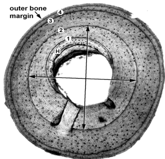
FIG. 1. Cross section of the femur diaphysis of Lacerta agilis boemica (adult male from Kuli). Ehrlich hematoxylin; magnification: ob. 6.3, oc. 3.2. H - hatching line; 1-4 - LAGs (= resting lines) of consecutive hibernations; arrows inside the section show the minimal and the maximal diameters of the bone limited by LAG2.
