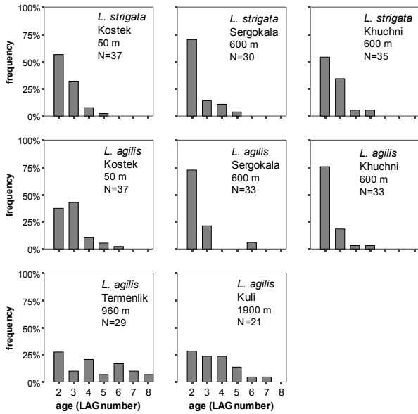
FIG. 2. Age (yr) distribution in adult samples of L. a. boeemica and L. strigata from five different localities of the eastern North Caucasus. Locality elevations are given within the plots.
