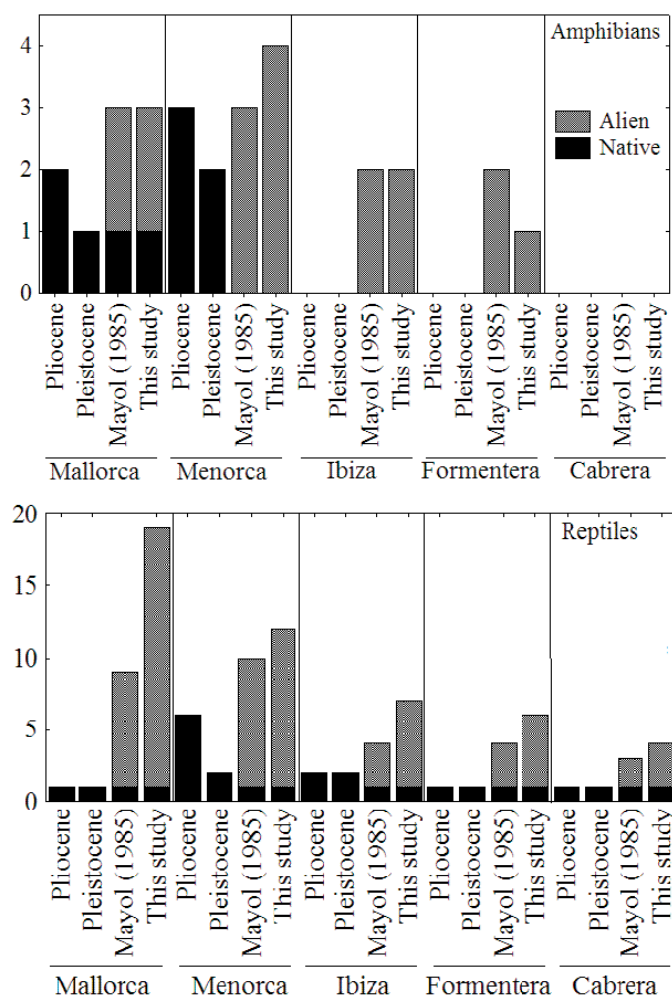
Fig. 1. Ancient and recent changes in the Balearic terrestrial herpetofauna.
