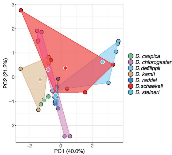
Figure 6. Principal component analysis of the meristic data.
