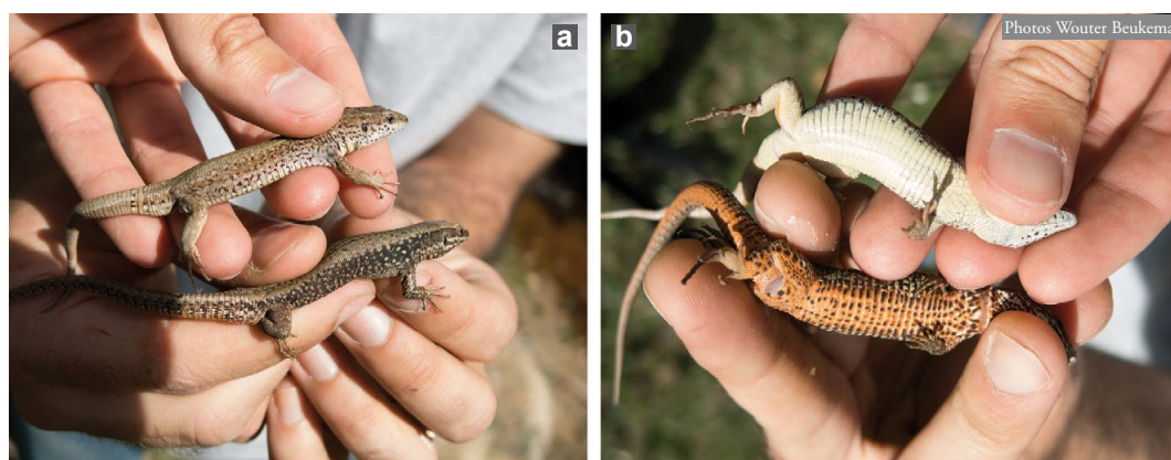
Figure 1: Dorsolateral a) and ventral b) views of Podarcis liolepis (top) and Podarcis muralis (bottom) found syntopically in Sierra de Urbión, Soria.
